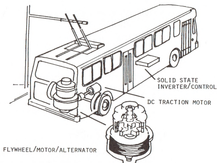
THIS TRANSIT BUS WITH A FLYWHEEL-ELECTRIC PROPULSION SYSTEM IS NOW UNDER DEVELOPMENT.
